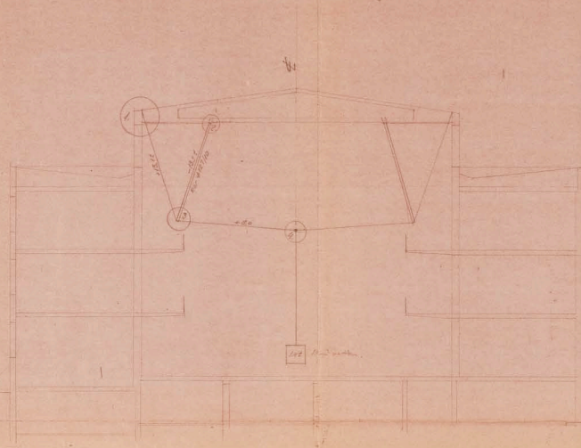
Settling on truss showing tensioning order for cables. 100
